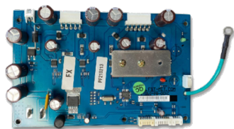
SHIATSULOGIC FX MASSAGE CHAIR - PCB CONTROL BOX
